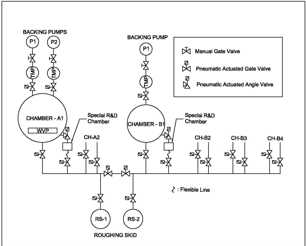
Fig.B1/1: Vacuum System schematic (Rev 01)
